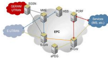
FIGURE 1. LTE Architecture [1]
