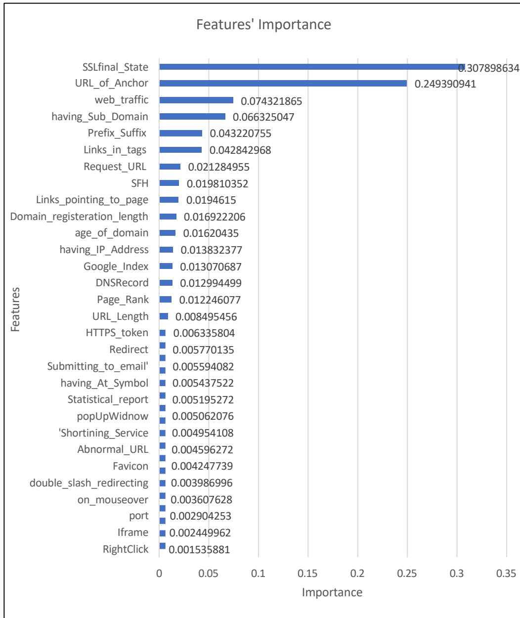
Figure 5: Feature importance rank and scores
