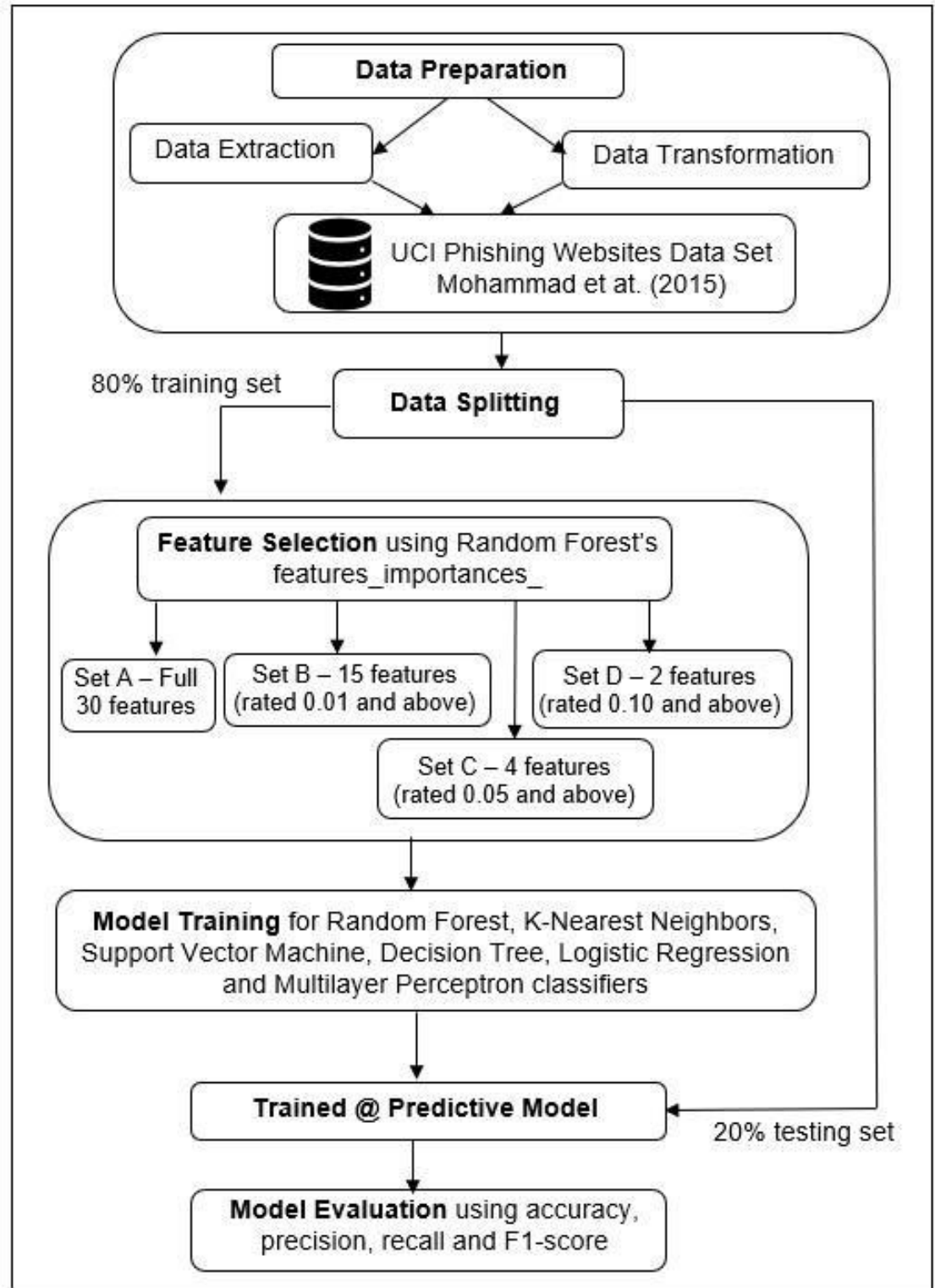
Figure 4: Proposed detection framework model
