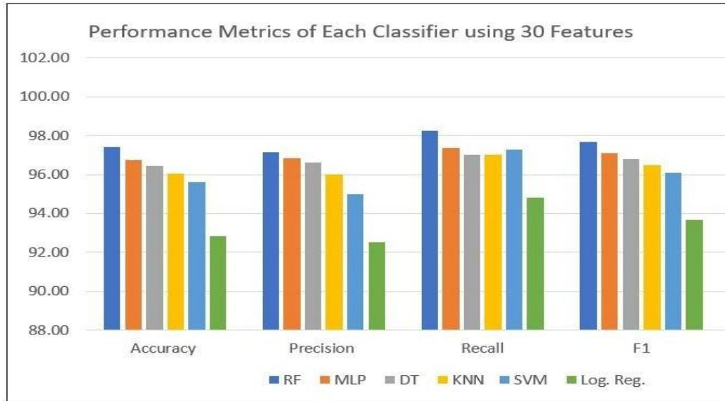
Figure 7: Performance metrics of classifiers using 30 features
