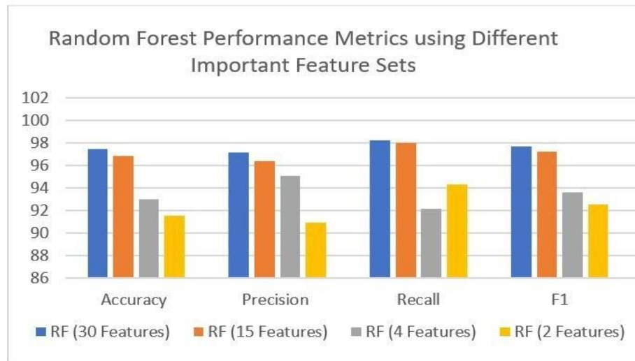
Figure 8: Performance metrics of classifiers using different feature sets
