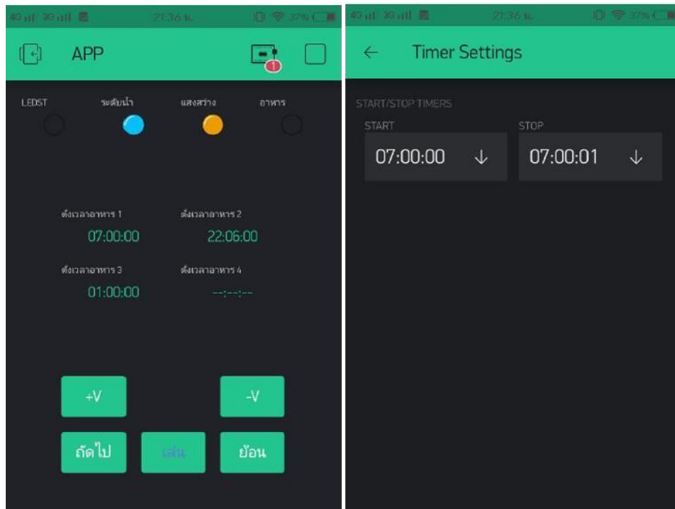
Figure 5: Blynk application
