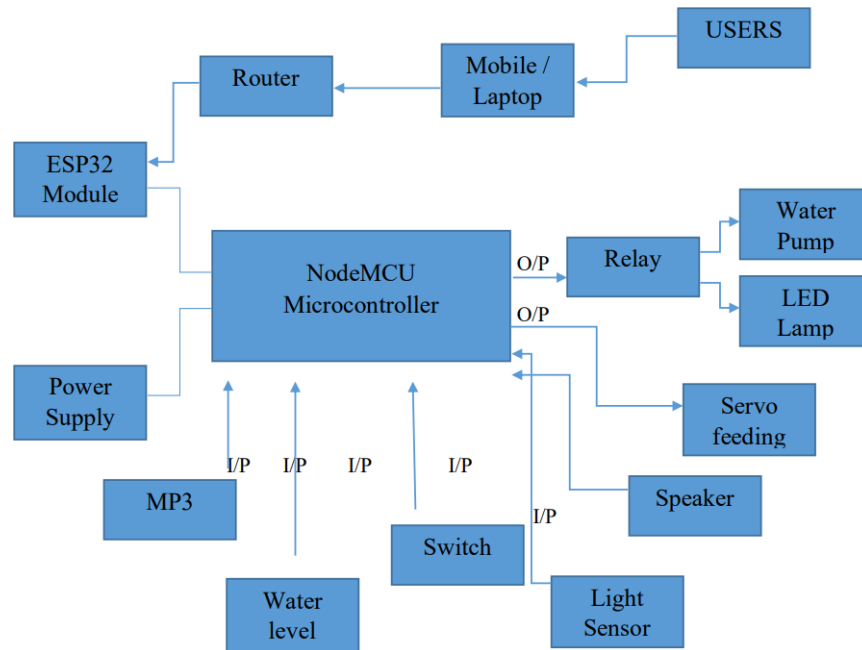
Figure 3: Functional Block Diagram of the System
